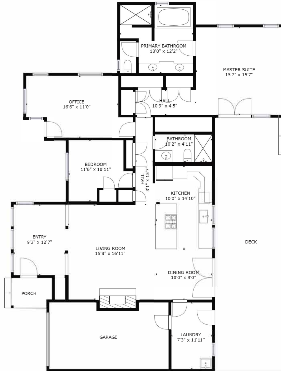
FLOOR 1
